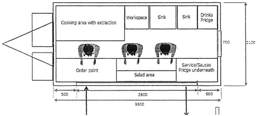
TRAILER INFORMATION: Kebab Trailer Model: 1-3.5m Trailer Dual Axle Floor Plan - Mehmet Ozer
